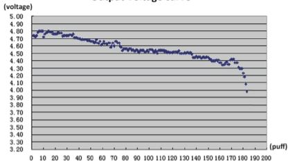
Output Voltage curve
